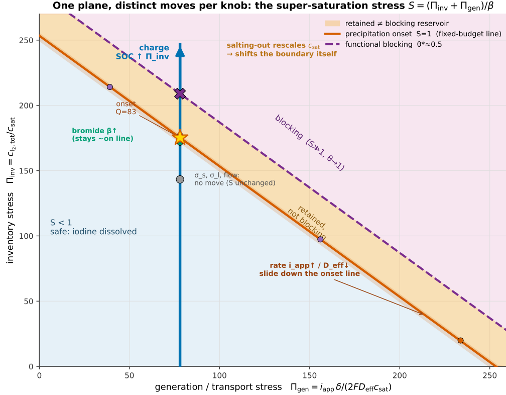
Figure 11: One plane, distinct moves per knob. The dimensionless knob phase plane. Axes are the generation/transport stress \Pi_{\text{gen}} = i_{\text{app}} \delta / (2FD_{\text{eff}} c_{\text{sat}}) and the inventory stress \Pi_{\text{inv}} = c_{\text{I}_2, \text{tot}} / c_{\text{sat}} , read directly from the solved surface field (at Q = 0 the oxidized inventory vanishes, so the surface total fixes \Pi_{\text{gen}} ). The orange line is the precipitation onset where the solved free monomer saturates ( S = 1 ); it is a nearly fixed budget line, \Pi_{\text{gen}} + \Pi_{\text{inv}} \approx 253 , because the buffer at onset is almost constant across cells ( \beta \approx 760 ), shown as a thin band for that small spread. (The larger \beta collapse 1263 \rightarrow 554 occurs along a charge trajectory and is what lifts S to onset; it is not the width of the boundary.) The dashed line is functional blocking ( \theta_{\text{eff}} = 0.5 ) and the amber strip between is the retained-not-blocking reservoir ( \Delta Q \approx 17 \text{ mA h cm}^{-2} ). The blue arrow is the baseline charge trajectory, climbing in \Pi_{\text{inv}} and crossing onset at Q = 83 . Coloured points are the solved precipitation-onset states of the rate, compression, bromide and diffusivity families; they collapse onto the one onset line — the geometric content of the organizing coordinate, each within-electrolyte knob acting on S_{\text{base}} through the node it perturbs. Salting-out instead rescales c_{\text{sat}} and shifts the boundary itself (off this fixed- c_{\text{sat}} plane); electronic and electrolyte conductivity and flow do not move the operating point (grey dot). The solved field references the free monomer at c_{\text{sat}}/3 (the slope-3.00 normalization of Fig. 8b); the onset locus is plotted in that solved convention.
