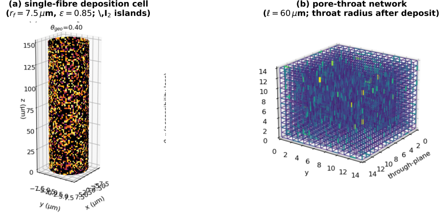
Figure 4: The mesoscale models. (a) The battery-calibrated single-fibre deposition cell ( r_f = 7.5 \mu\text{m} , \varepsilon = 0.85 ) with stochastically nucleated I_2 islands, and (b) the pore-throat network after deposit, whose accessibility \theta_{\text{eff}}(\varepsilon_s) and permeability K(\varepsilon_s) closures (Fig. 5) are handed to the continuum solve. At the operating solid load the deposit remains sub-monolayer islands rather than a continuous film, consistent with the percolation-limited accessibility loss.
