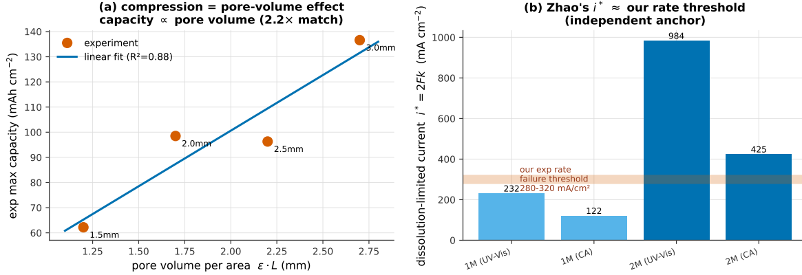
Figure 9: Dissolution-limited magnitude, externally anchored. (a) The geometric limit Q_f \propto \varepsilon L ; full-cell capacities (reported separately) are shown only as an external consistency check. (b) The dissolution-limited current i^* = 2Fk for the rate constants of Zhao et al. [16]; the bars span the reported k at the two iodide concentrations and the two estimation methods, and the body uses the i^* \approx 232\text{--}425 mA cm -2 range from k = (1.2\text{--}2.2) \times 10^{-6} mol cm -2 s -1 (we are at 2 M I - ).
