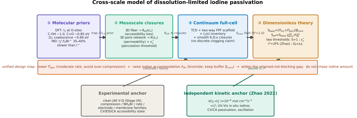
Figure 2: Cross-scale model. Molecular priors (DFT trapping, MD transport) set the closures; 3D fiber/pore-network models supply the accessibility \theta_{eff}(\epsilon_s) and permeability K(\epsilon_s) closures and accessibility/permeability cross-checks; the continuum model integrates them using a calibrated, closure-conditioned blocking threshold \epsilon_s^* , and the reduced stress framework distills the model stack into design rules. The experimental families and the independent dissolution kinetics provide external anchors and scope checks for the chain.
