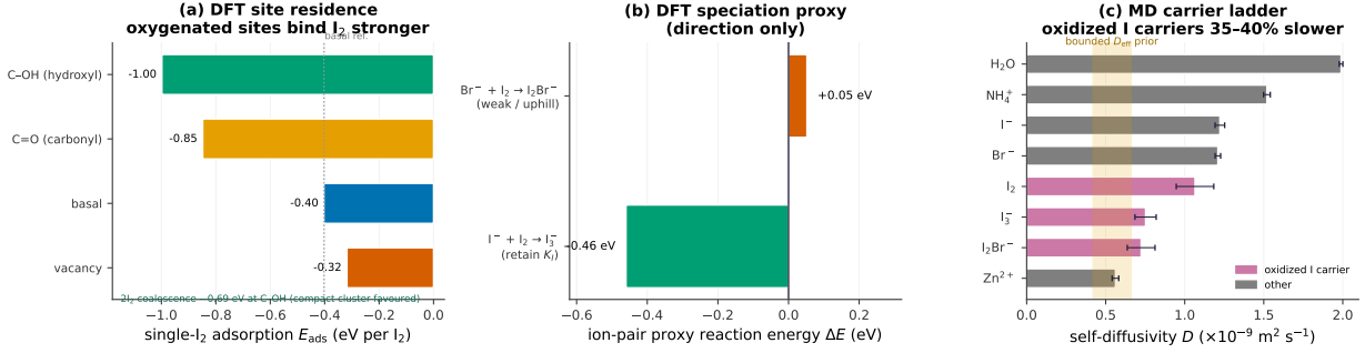
Figure 3: Molecular priors (bounds, not rates). (a) DFT single-I 2 adsorption energies (basal -0.40 , carbonyl -0.85 , hydroxyl -1.00 , vacancy -0.32 eV): oxygenated defects bind I 2 roughly twice as strongly as basal, and a 2I 2 coalescence of -0.69 eV at C-OH favours compact clusters. (b) DFT speciation proxy (direction only): the I 3 - branch is downhill, the I 2 Br - branch borderline-uphill. (c) MD carrier diffusivities: the oxidised carriers I 3 - and I 2 Br - are 38–41% slower than I - (neutral I 2 only \sim 12\% ); shaded band is the low-end D_{\text{eff}} prior.
