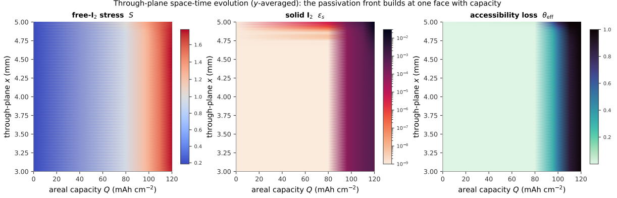
Figure 6: Through-plane space-time evolution ( y -averaged): the passivation front (free- I_2 stress, solid I_2 , accessibility loss) builds at one face as capacity increases.
