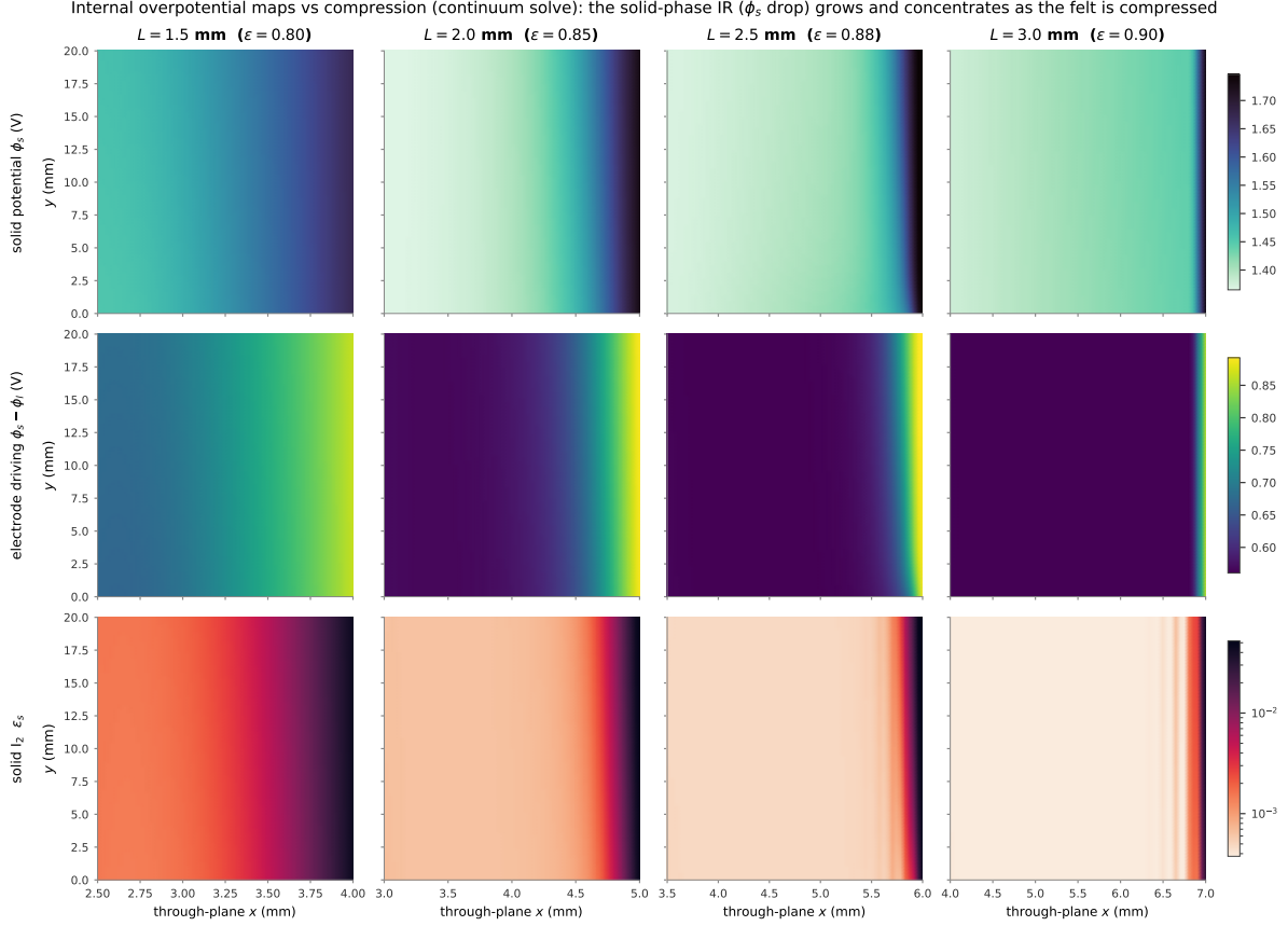
Figure 12: Internal overpotential maps vs compression (native continuum solve): rows show the solid-phase potential ( \phi_s ) drop, the electrode driving potential ( \phi_s - \phi_\ell ) and the solid I_2 fraction ( \epsilon_s ) across L = 1.5 – 3.0 mm; the electronic/contact penalty grows and concentrates toward the collector as the felt is compressed.
