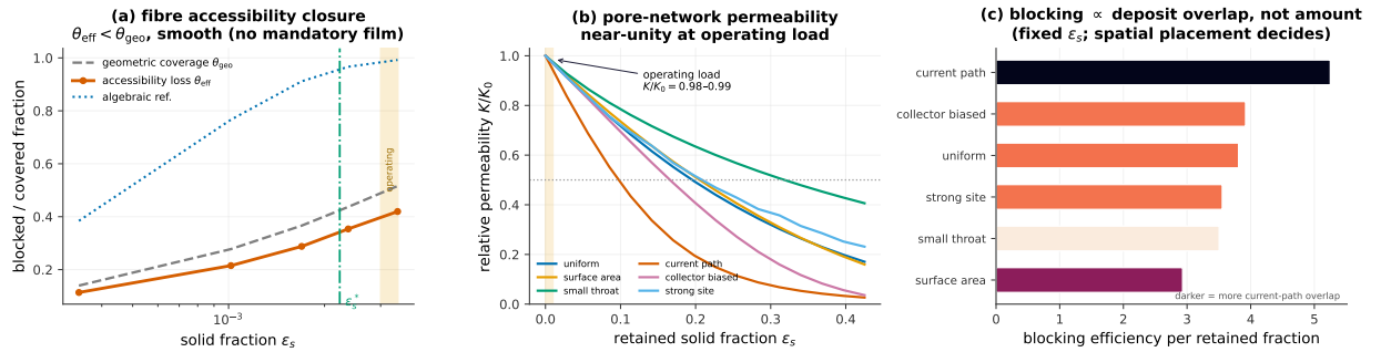
Figure 5: Mesoscale closures (calibrated, postprocessed). (a) Fibre accessibility closure \theta_{\text{eff}}(\varepsilon_s) lies below the geometric coverage and declines smoothly (no mandatory film); \varepsilon_s^* is the percolation threshold. (b) Pore-network relative permeability K(\varepsilon_s) for six deposit-placement laws stays near unity at the operating load; halving it needs 30–100 \times more solid. (c) Blocking efficiency is set by the spatial overlap of deposit, not its amount.
