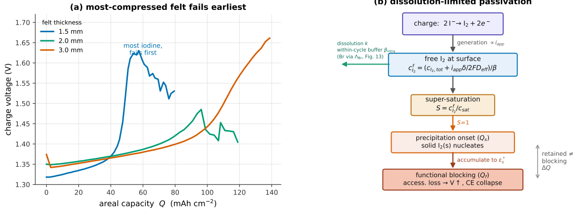
Figure 1: Iodine amount is not the penalty; functional blockage is a state transition. (a) Charge curves from a compression series at fixed current density: the most-compressed felt reaches voltage runaway at the lowest usable capacity, even though the model predicts more local retained iodine. This motivates, but does not by itself prove, the separation between retained iodine and blocking iodine. (b) Mechanism formalized in Sec. 2. Charge generates oxidized iodine; within a given electrolyte the within-cycle buffer \beta_{\text{intra}} buffers the free- \text{I}_2 monomer and sets the baseline surface stress S_{\text{base}} . When S_{\text{base}} reaches unity, native \text{I}_2(\text{s}) is retained (precipitation onset Q_s ); functional blocking ( Q_f ) occurs only after the retained solid crosses the accessibility threshold \varepsilon_s^* , and the gap \Delta Q is retained-but-not-blocking iodine. Cross-composition bromide effects are carried separately by the iodine-accommodation factor \Lambda_{\text{Br}}^{\text{rel}} (Fig. 13).
