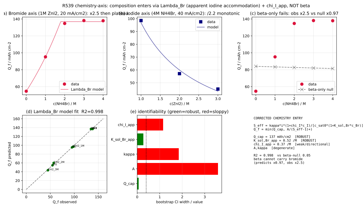
Figure 13: Experimental chemistry axis and the bromide-accommodation correction. (a) Areal capacity vs. supporting bromide (1 M ZnI_2 , 20 mA cm -2 ): \sim 2.5\times rise saturating by 2–3 M. (b) vs. ZnI_2 (4 M NH_4Br , 40 mA cm -2 ): monotonic \div 2.2 decline. (c) the \beta -only stress predicts a near-flat bromide response (0.97 \times ) against the observed 2.5 \times . (d) the \Lambda_{Br} model fits both axes, R^2 = 0.998 . (e) bootstrap identifiability: Q_{cap} and K_{sol,Br}^{app} robust; A , \kappa , \chi_I^{app} sloppy. Capacities are max-deliverable from raw .ndax; full cells 4 cm 2 , three-electrode tests (Ag/AgCl, positive felt) 1 cm 2 .
