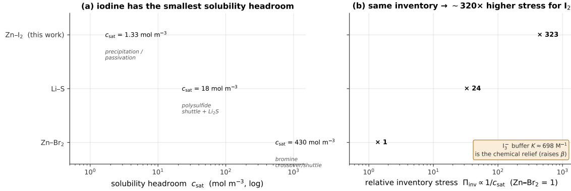
Figure 14: Cross-chemistry universality of dissolution-limited passivation. (a) Solubility headroom c_{\text{sat}} of the condensable intermediate for three conversion chemistries (aqueous for I 2 /Br 2 ; an illustrative non-aqueous dissolved-sulfur model cap for Li-S): I 2 /ZnI 2 (1.33 mol m -3 [24]), Li-S dissolved sulfur ( \approx 18 \text{ mol m}^{-3} [46]) and Br 2 /ZnBr 2 (430 mol m -3 [47]). (b) The implied inventory stress \Pi_{\text{inv}} \propto 1/c_{\text{sat}} at fixed oxidized inventory (normalized to ZnBr 2 ): iodine bears \sim 320\times the stress of bromine and \sim 14\times that of Li-S, the structural reason ZnI 2 is uniquely precipitation/passivation-limited. The I 3 - complexation buffer ( K \approx 698 \text{ M}^{-1} [12]) is the chemical relief identified by the buffer \beta . Values are external literature data, not model outputs.
