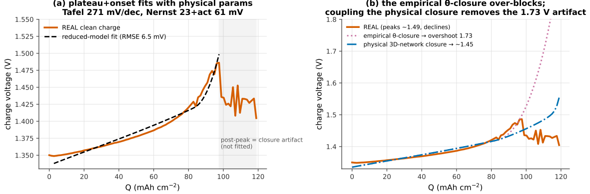
Figure 10: Stage-I/II voltage observable layer. A reduced observable layer (not the native COMSOL terminal voltage) aligns the normal and rising portions of the clean charge curve with the state clock. (a) The reduced Butler–Volmer model (Eq. 18) fits the real pre-failure charge curve to 6.5 mV; the rise is dominated by iodide depletion. (b) The empirical accessibility closure over-blocks past the real peak (voltage overshoot); coupling the physical mesoscale closure removes the artifact—no coalesced film is required.
