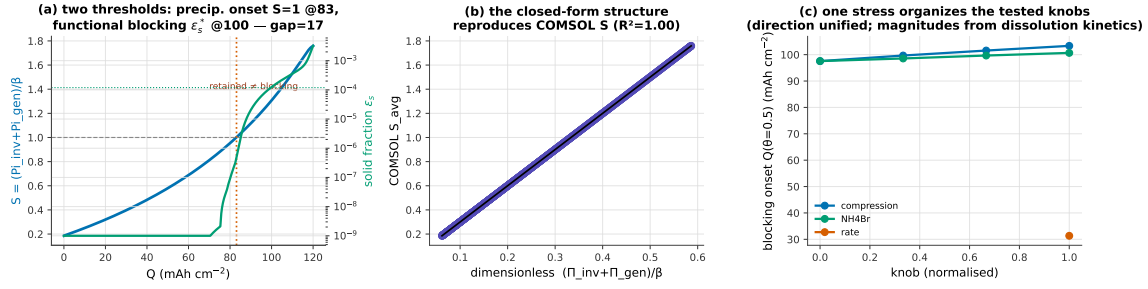
Figure 8: Dimensionless theory of dissolution-limited passivation. (a) The super-saturation stress S_{\text{base}} = (\Pi_{\text{inv}} + \Pi_{\text{gen}})/\beta_{\text{intra}} crosses unity (precipitation onset, Q_s ) well before the solid fraction reaches the functional-blocking threshold \varepsilon_s^* ( Q_f ); the gap is the retained-but-not-blocking capacity. (b) The closed form reproduces the continuum-model super-saturation field ( R^2 = 1.000 , up to a constant normalization). (c) The stress coordinate organizes the tested operating/design knobs by the mechanism node each perturbs.
