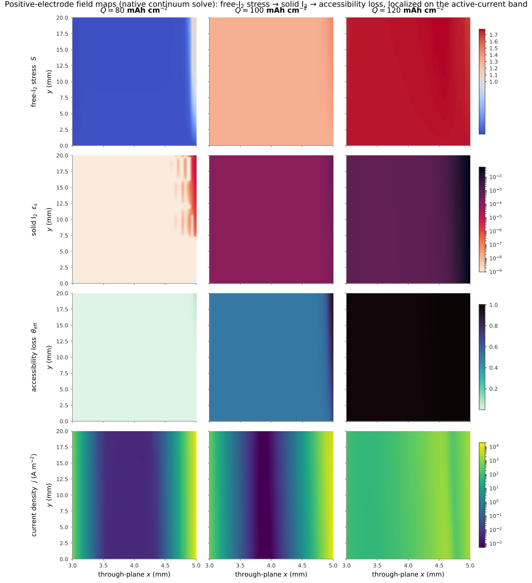
Figure 7: Native two-dimensional field maps of the positive electrode (free-I 2 stress S , solid I 2 \varepsilon_s , accessibility loss \theta_{\text{eff}} , total current density j ) at Q = 80/100/120 \text{ mAh cm}^{-2} . Solid iodine and current localize in a thin band at one face while S stays a smooth through-plane gradient.
